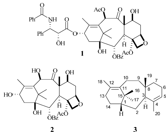
FIGURE 1. Structures of taxane diterpenes.
