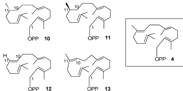
FIGURE 2. Analogues 10–13 used in this study, which are dissimilar to GGPP 4 at the \Delta^{10} double bond.
