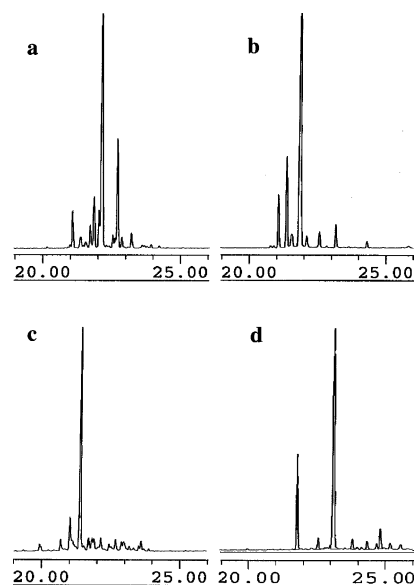
FIGURE 3. GCMS analyses, displaying the total ion current of the hydrocarbon products from the incubation of taxadiene synthase with analogues 10 (panel a), 11 (panel b), 12 (panel c), and 13 (panel d). GCMS analyses were performed using a 30 M, 0.25 mm i.d., 0.25 μM DB-5MS column, programmed 120 °C for 2.00 min, to 280 °C at 5 °C/min, final time 15 min. In control experiments, incubation of analogues 10 – 13 with BL21/DE3/plysS (which does not encode taxadiene synthase) failed to give any hydrocarbon products on TLC.
